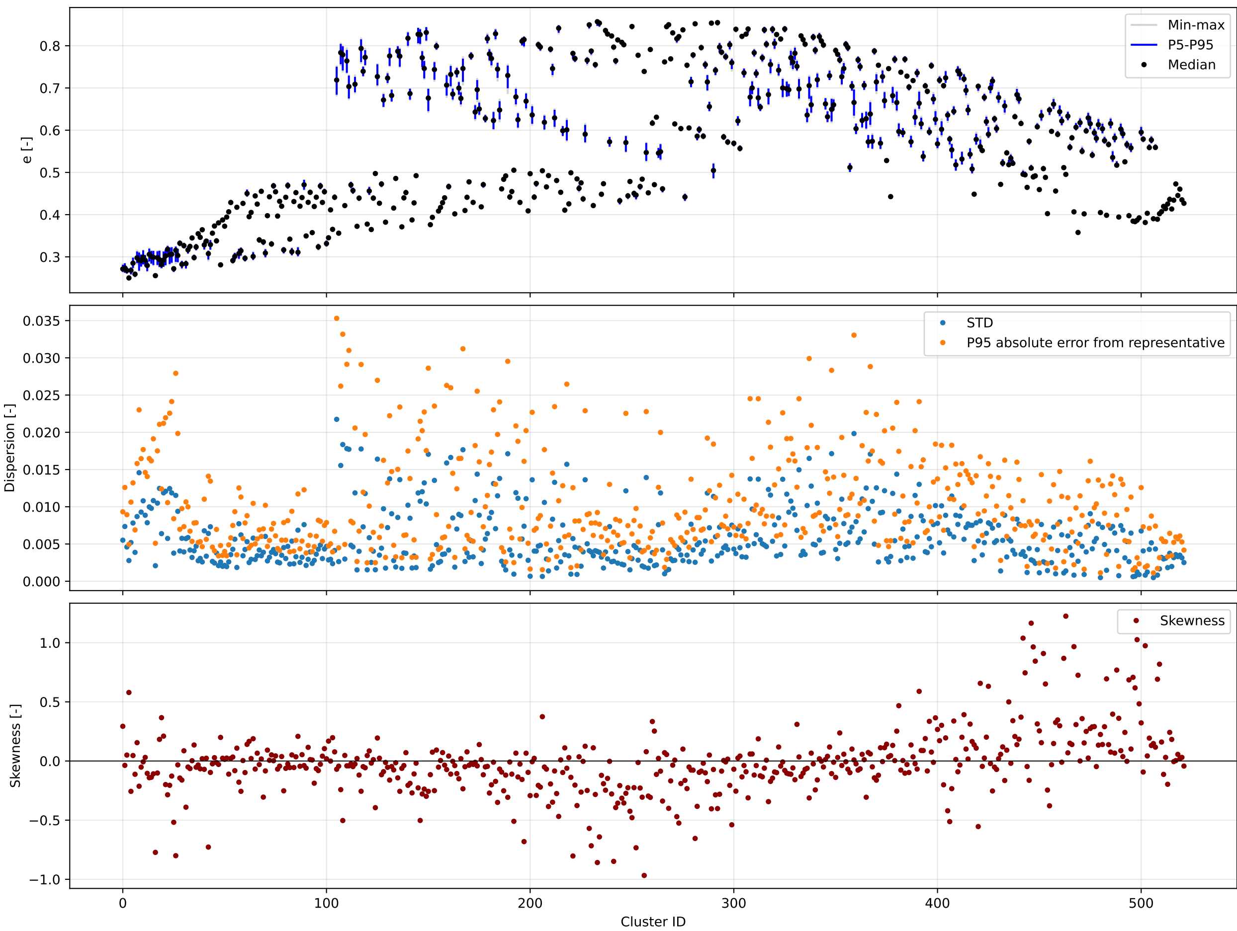
K=522 | backward | e | valid=59218/59218 assigned
